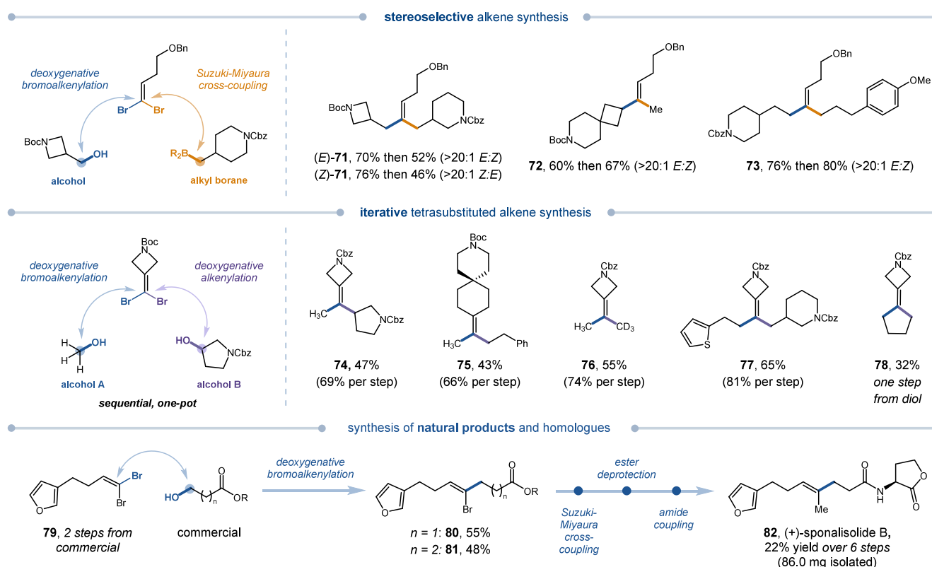
Figure 2. Sequential strategies toward piecewise assembly of multisubstituted alkenes. (See the Supporting Information for experimental details.)
