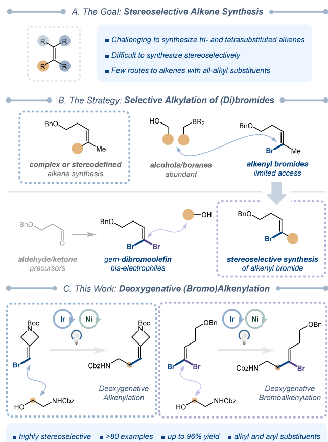
Figure 1. Strategic approach to stereoselective multisubstituted alkene synthesis.
