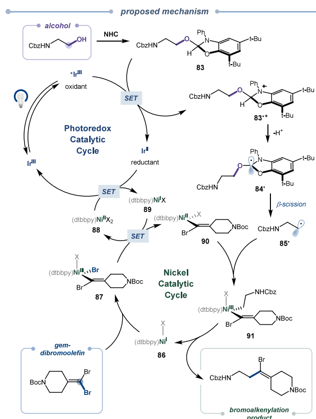
Figure 3. Proposed mechanism.
