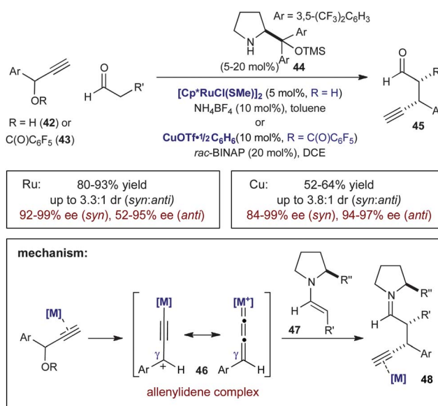
Scheme 13 Nishibayashi's enantioselective \alpha -propargylation of aldehydes via enamine and transition metal catalysis.
