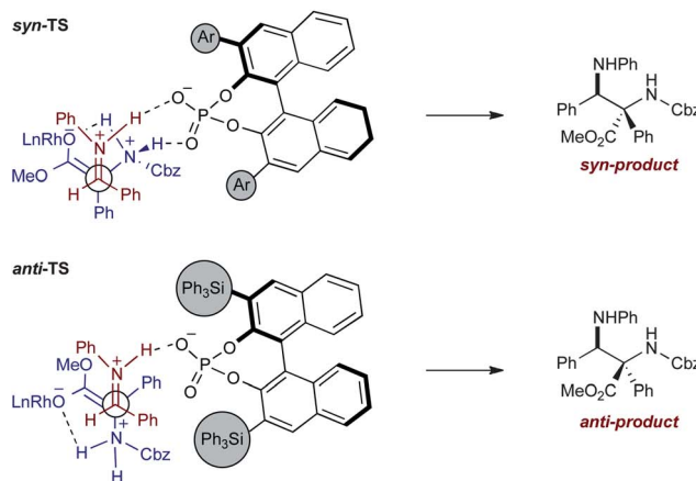
Scheme 36 The three-component coupling of diazoacetates, carbamates, and imines using a chiral Brønsted acid and \text{Rh}_2(\text{OAc})_4 .
