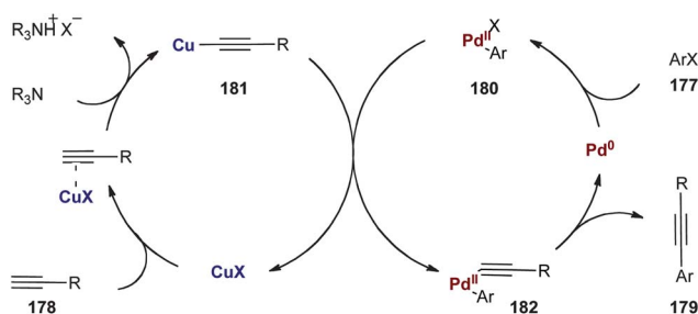
Scheme 44 The Sonogashira coupling reaction first disclosed in 1975 by Sonogashira, Tohda, and Hagihara.
