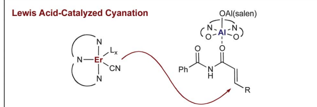
Scheme 27 Jacobsen's conjugate cyanation of unsaturated imides.
