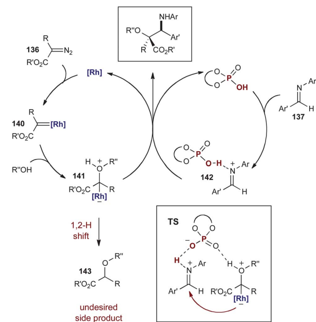
Scheme 34 Mechanism of the three-component coupling of diazoacetates, alcohols, and imines via rhodium- and Brønsted acid catalysis.
