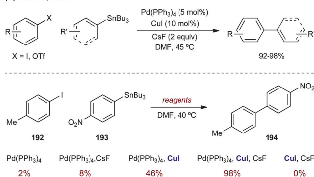
Scheme 46 Palladium- and copper-catalyzed Stille coupling reactions.
