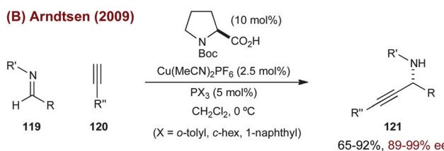
Scheme 29 Asymmetric synthesis of propargylic amines via the merger of transition metal catalysis with Brønsted acid catalysis.
